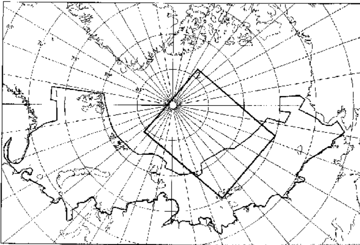
Figure 1. Portions of the Arctic Ocean seabed that are included in the integrated bathymetric grid produced at VNIIOkeangeologia. 1: Northern Eurasian Shelf. 2: Central Arctic Basin. (Maschenkov)
