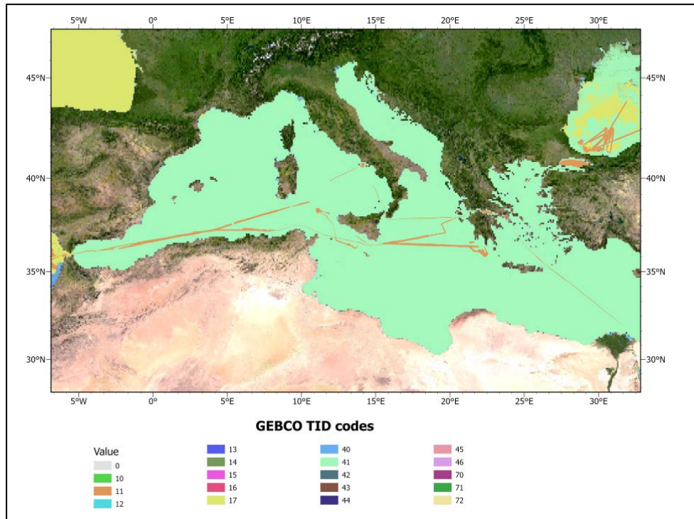
Figure 1. GEBCO_2023 TID Grid for the Mediterranean Sea region showing regions wrongly coded as TID 41
