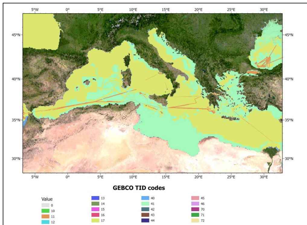
Figure 2. Revised TID coding for GEBCO_2023 for the Mediterranean Sea
